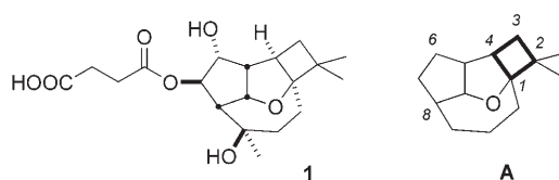
Scheme 1. Structure of punctaporonin C ( 1 ) and its core skeleton A with the cyclobutane ring highlighted.
