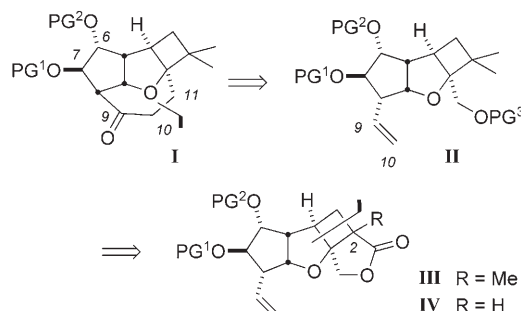
Scheme 2. Retrosynthetic analysis of punctaporonin C ( 1 ).
