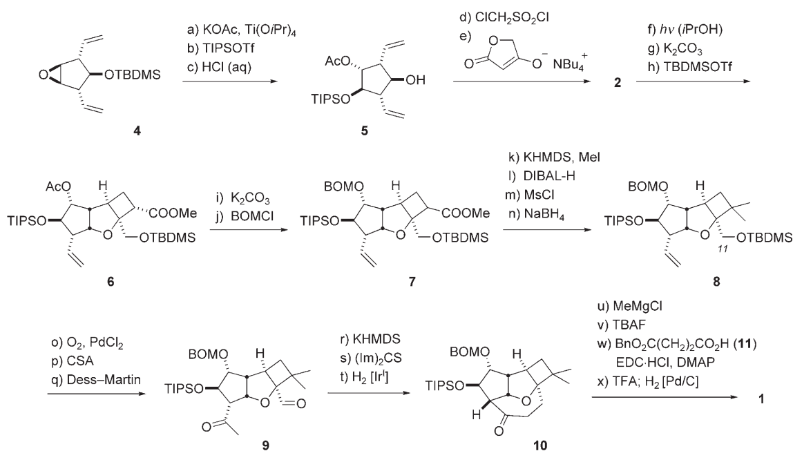
Scheme 4. Total synthesis of (±)-punctaporonin C ( 1 ): a) KOAc, \text{Ti}(\text{O}i\text{Pr})_4 (50 mol %), HOAc, 90^\circ\text{C} , 9 h, 76 %; b) TIPSOTf, 2,6-lutidine, \text{CH}_2\text{Cl}_2 , 0^\circ\text{C} , 3 h; c) HCl (aq), MeOH, 20^\circ\text{C} , 6 h, 91 % for 2 steps; d) chloromethanesulfonyl chloride, pyridine, -10^\circ\text{C} , 4 h, 95 %; e) tetrabutylammonium tetronate, THF, 67^\circ\text{C} , 20 h, 80 %; f) h\nu , i PrOH, -75^\circ\text{C} , 1.5 h, d.r. 75:25; g) \text{K}_2\text{CO}_3 (20 mol %), MeOH, -20^\circ\text{C} , 2 h; h) TBDMSOTf, 2,6-lutidine, \text{CH}_2\text{Cl}_2 , -20^\circ\text{C} , 3 h, 60 % for 3 steps; i) \text{K}_2\text{CO}_3 , MeOH, 20^\circ\text{C} , 3 days, 80 %; j) BOMCl, TBAI, \text{NETiPr}_2 , \text{ClCH}_2\text{CH}_2\text{Cl} , 50^\circ\text{C} , 36 h, 80 %; k) KHMDS, MeI, THF, -40 \rightarrow -78^\circ\text{C} , 3 h, d.r. 80:20, 56 %; l) DIBAL-H, THF, -78^\circ\text{C} , 4 h, 81 %; m) MsCl, \text{NEt}_3 , \text{CH}_2\text{Cl}_2 , -20^\circ\text{C} , 4 h, quantitative; n) \text{NaBH}_4 , DMPU, 75^\circ\text{C} , 24 h, 77 %; o) \text{O}_2 , \text{PdCl}_2 , CuCl, DMF/ \text{H}_2\text{O} (10:1), 20^\circ\text{C} , 4 days, 94 %; p) CSA (50 mol %), \text{CH}_2\text{Cl}_2/\text{MeOH} (10:1), 20^\circ\text{C} , 24 h, 91 %; q) Dess–Martin, \text{CH}_2\text{Cl}_2 , 20^\circ\text{C} , 1 h, quantitative; r) KHMDS, THF, -78 \rightarrow -40^\circ\text{C} , 30 min, 56 %; s) (\text{Im})_2\text{CS} , DMAP, \text{CH}_2\text{Cl}_2 , 20 \rightarrow 40^\circ\text{C} , 16 h, quantitative; t) \text{H}_2 , [\text{Ir}(\text{cod})\text{P}(\text{c}\text{-C}_6\text{H}_{11})_3(\text{py})]\text{PF}_6 (10 mol %), \text{CH}_2\text{Cl}_2 , 20^\circ\text{C} , 2 h, 94 %; u) \text{MeMgCl} , \text{Et}_2\text{O} , 20^\circ\text{C} , 16 h, d.r. 87:13, 83 %; v) TBAF, THF, 0^\circ\text{C} , 3 h, 89 %; w) \text{BnO}_2\text{C}(\text{CH}_2)_2\text{CO}_2\text{H} ( 11 ), EDC-HCl, DMAP, \text{CH}_2\text{Cl}_2 , 20^\circ\text{C} , 16 h, 95 %; x) TFA, \text{CH}_2\text{Cl}_2 , 20^\circ\text{C} , 1.5 h; \text{H}_2 , Pd/C, MeOH/ethyl acetate (1:1), 20^\circ\text{C} , 16 h, 85 % for 2 steps. Bn = benzyl, BOMCl = benzyloxymethyl chloride, cod = 1,5-cyclooctadiene, CSA = camphorsulfonic acid, DIBAL-H = diisobutylaluminum hydride, DMAP = 4-dimethylaminopyridine, DMF = N,N -dimethylformamide, DMPU = 1,3-dimethyltetrahydropyrimidin-2(1 H )-one, EDC = N -ethyl- N' -(3-dimethylaminopropyl)carbodiimide, HMDS = hexamethyldisilazide, (\text{Im})_2\text{CS} = thiocarbonyldiimidazole, Ms = methanesulfonyl, py = pyridine, TBAF = tetrabutylammonium fluoride, TBAI = tetrabutylammonium iodide, Tf = trifluoromethanesulfonyl, TFA = trifluoroacetic acid.
