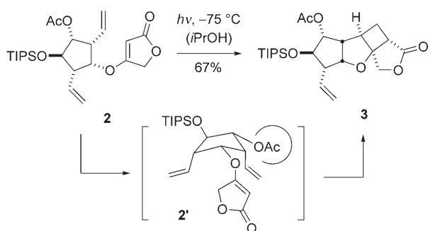
Scheme 3. Regio- and stereoselective [2+2] photocycloaddition of tetronate 2 to give 3 , with a depiction of the putative preferred conformation 2' . Reaction conditions: h\nu ( \lambda = 254 nm), i PrOH, -75^\circ\text{C} , 1.5 h, c = 7 mM.
